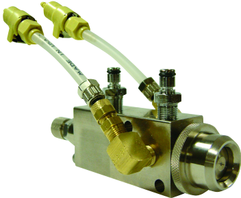
DS-20 Macro-Mini recirculating marker
